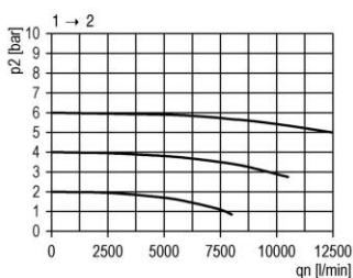
flow characteristic
